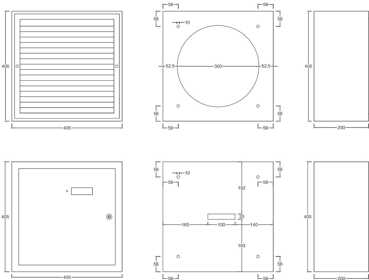
M500BJ, dimensioni macchina, 2D Model
